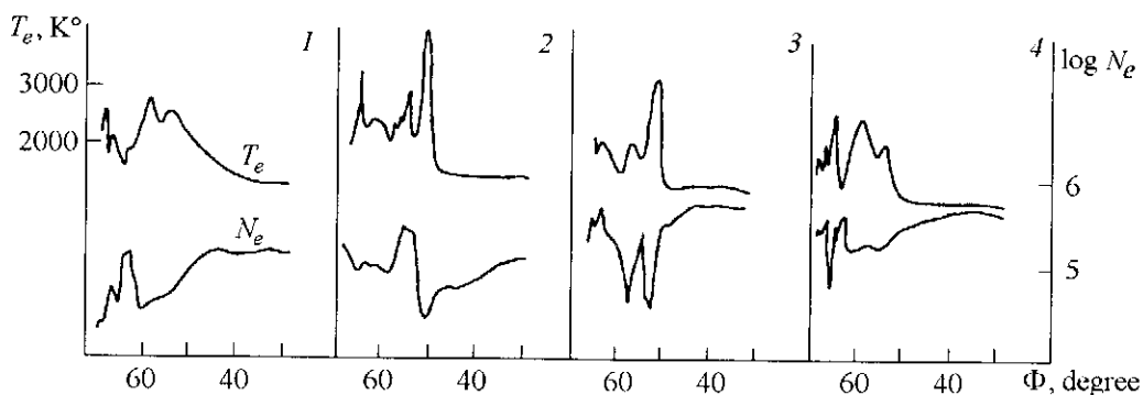
Figure 2. Latitude variations of N_e and T_e during the storm on July 26-27, 1979 for satellite passes indicated by 1, 2, 3, and 4, respectively, in Figure 1.
