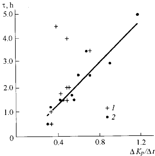
Figure 3. Delay \tau in response of a trough to Kp index variations as a function of the perturbation growth rate \Delta Kp/\Delta t ; 1, evening hours; and 2, near midnight and after midnight hours of local time.
