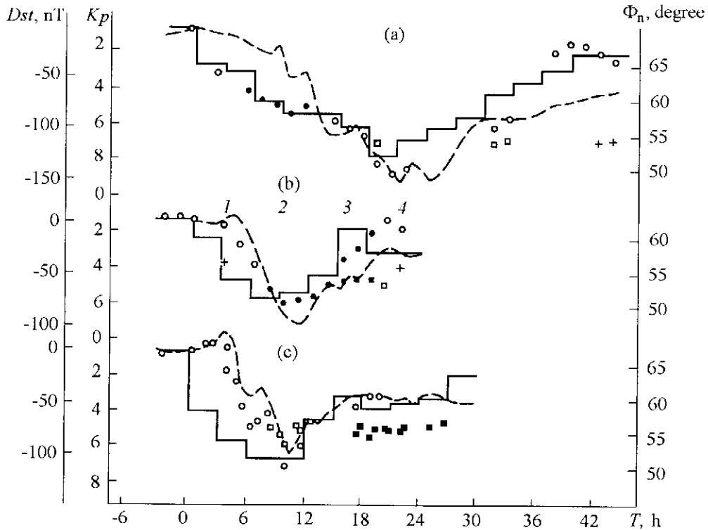
Figure 1. Variations in positions of troughs during three magnetic storms: (a) August 28-30, 1979, 1800-2000 MLT; (b) July 26-27, 1979, 2300-0100 MLT; and (c) March 21-22, 1979, 0300-0500 MLT. The solid lines show variations in the Kp index, dashed lines indicate Dst variations, circles show the main ionospheric trough; squares denote the ring ionospheric trough, solid circles show a narrow ionization trough, and crosses indicate the T_e peak.
